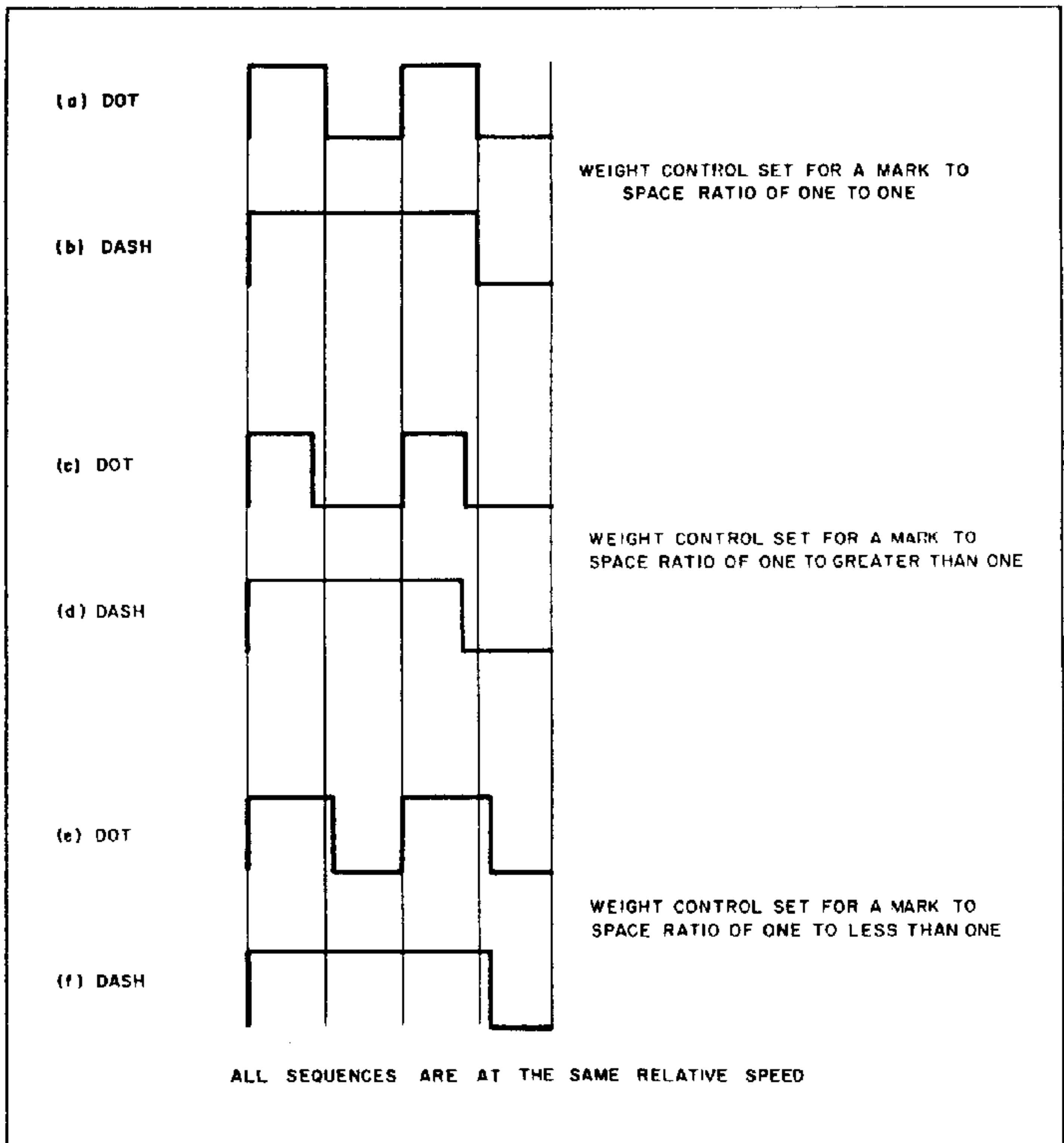
Figure 6. Dot-Dash-Space Relationship With Various Weight Control Settings.
