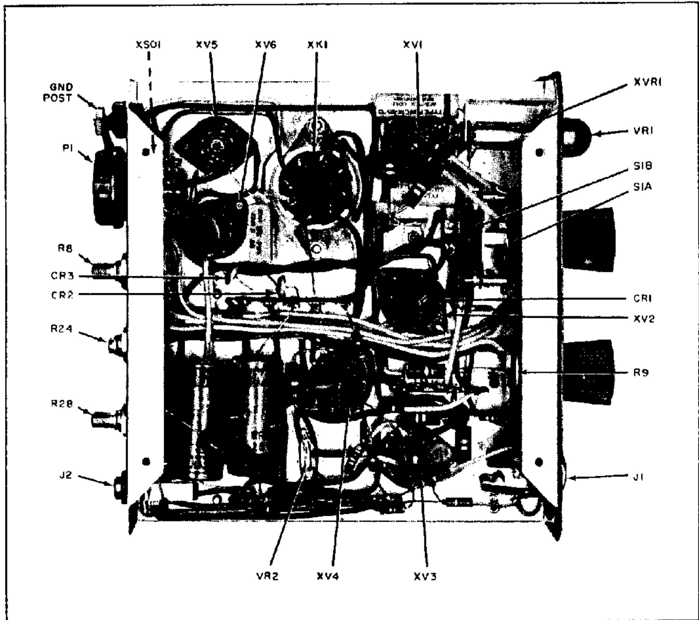
Figure 8. Model HA-1 Bottom Chassis View.
