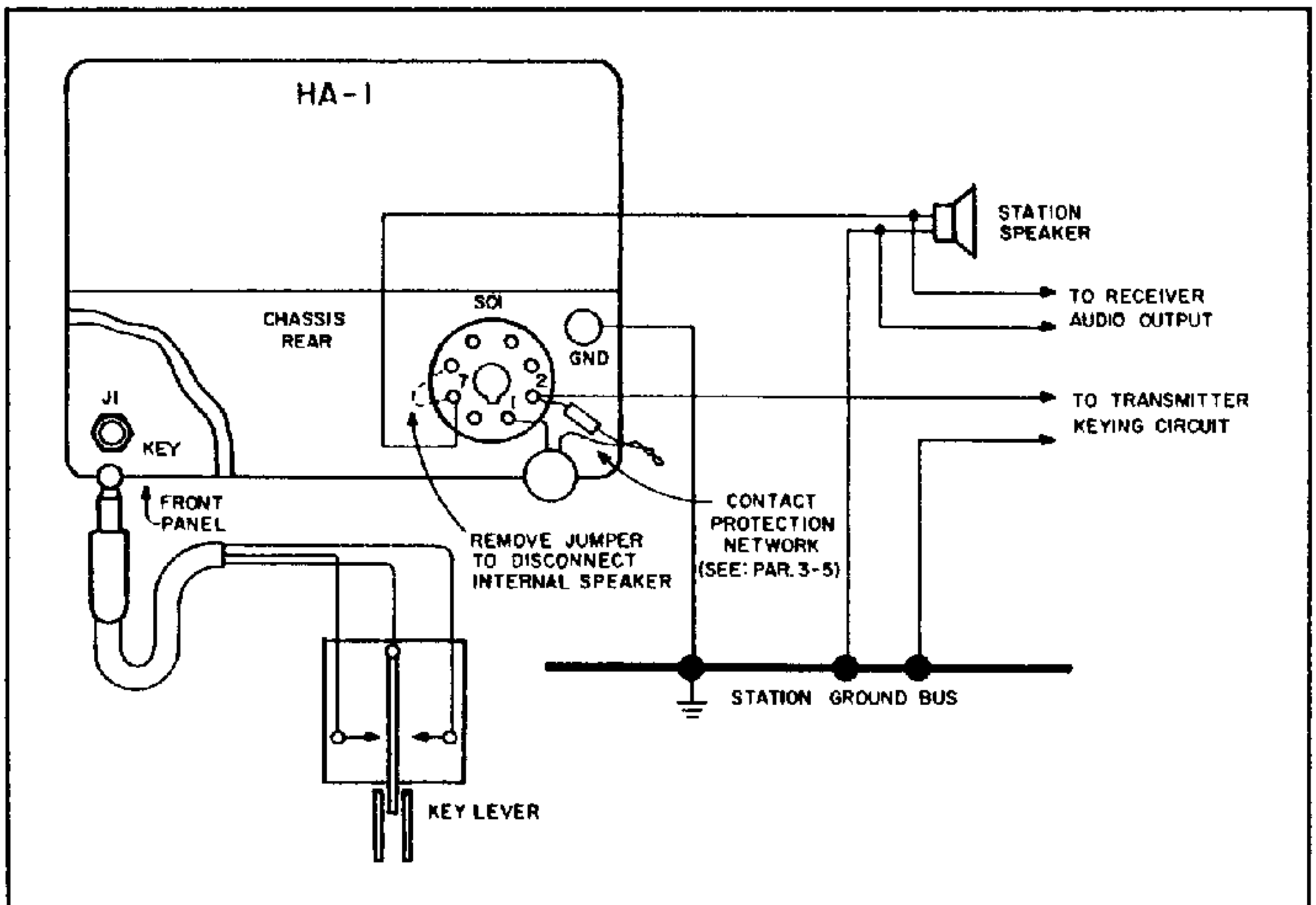
Figure 4. Typical Station Installation.
